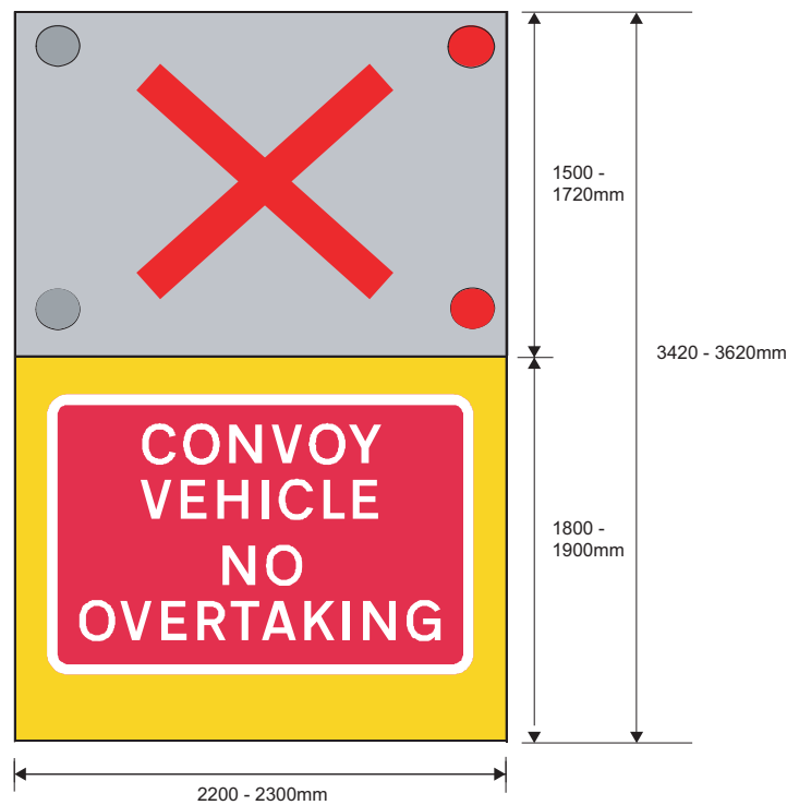
Figure 11.1 Closure vehicle sign
