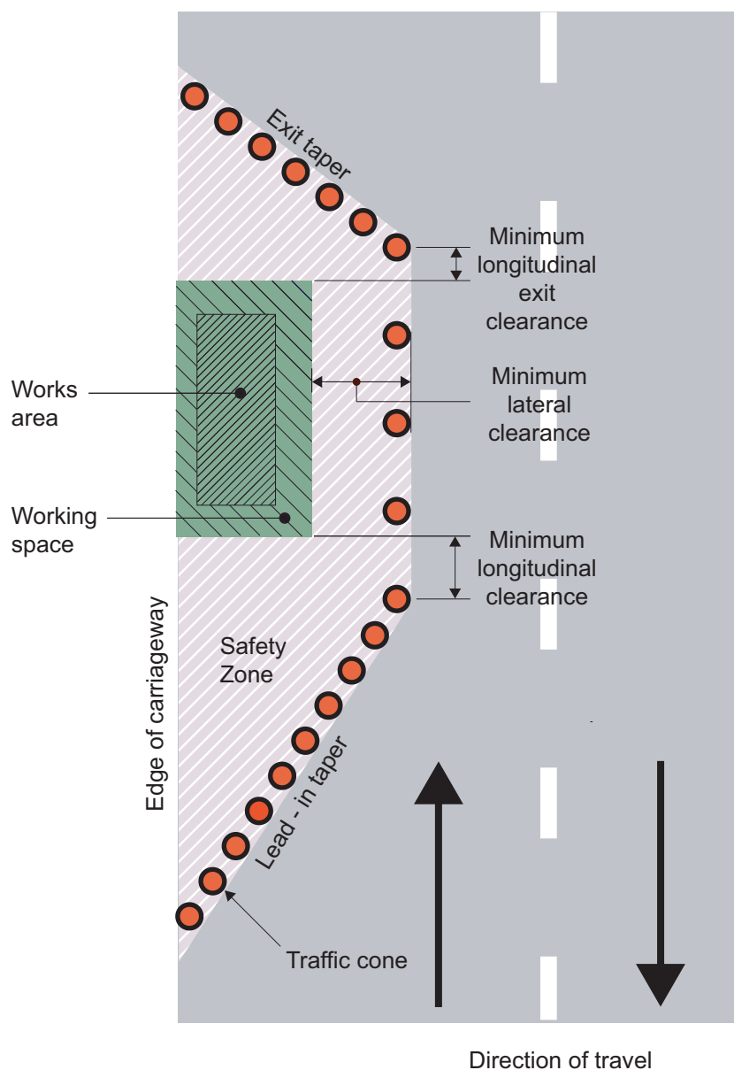
Figure 3.1 Safety zones – typical site layout
